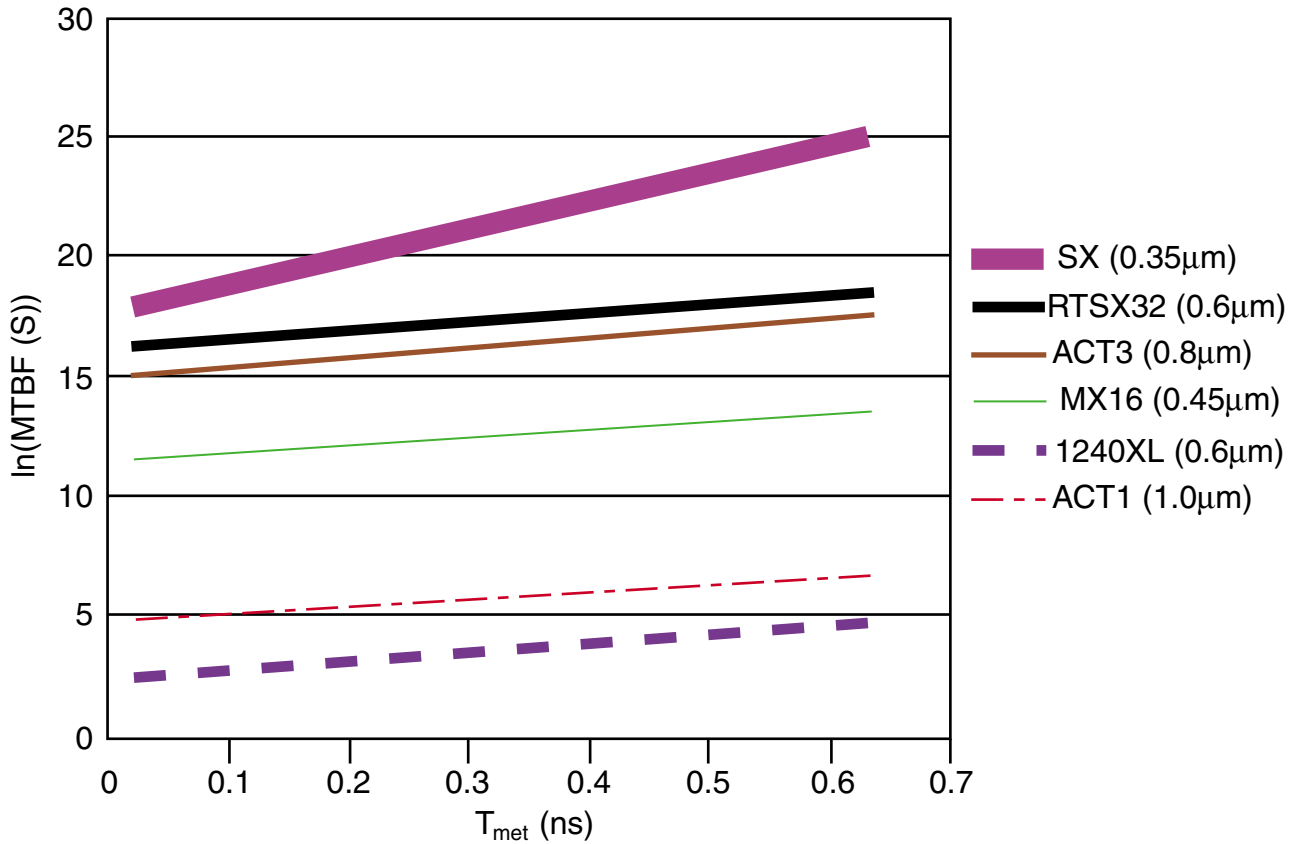
Figure 1 • Metastability Comparison of Actel FPGA Families
